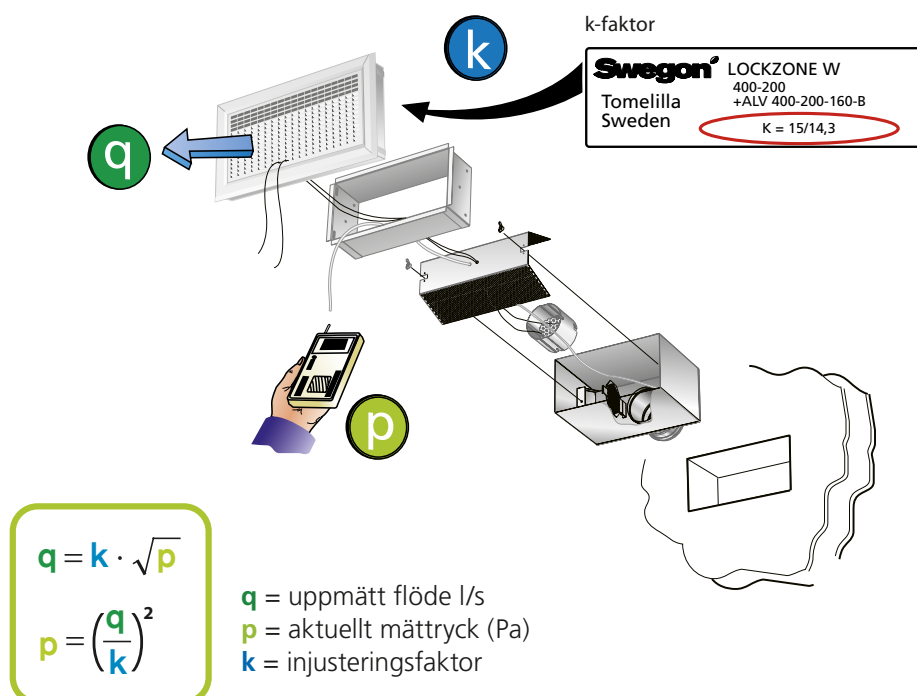
Figur 1. Montering. Injustering.
